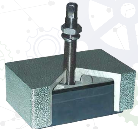
CUTAWAY VIEW OF IM-61 MOUNT
