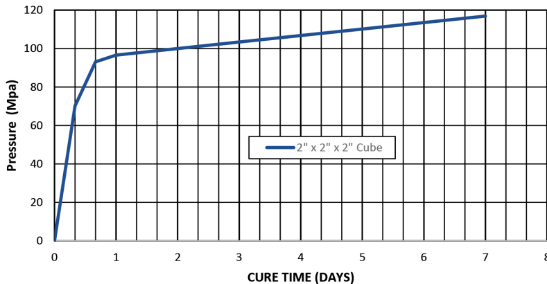
WTF-E V-100 EPOXY GROUT TYPICAL FIELD RESULTS
